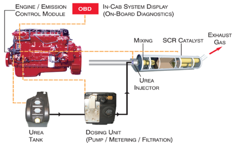
Fig 2. How an SCR system works
